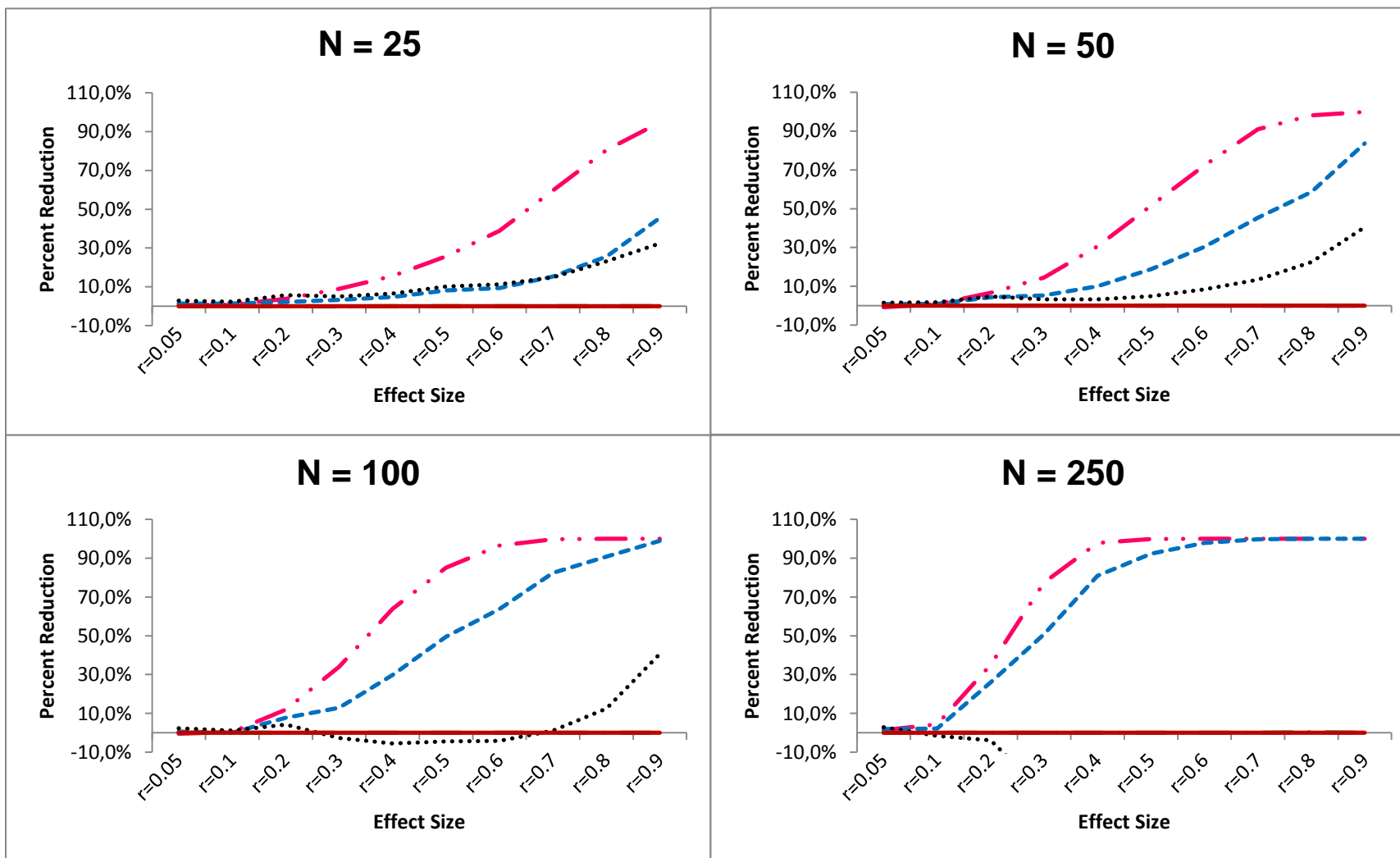
Figure 2. Type II Error Reduction Achieved by Transformation for Heavily Skewed Distributions
