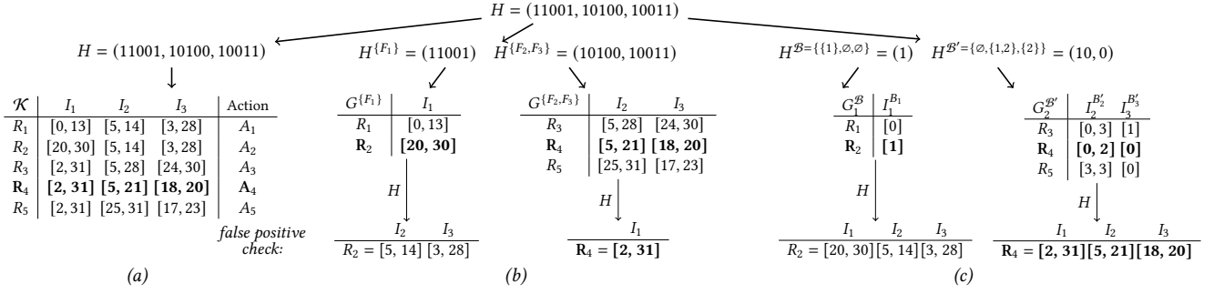
Figure 2: Multigroup representations our RR method vs. SAX-PAC [10]: (a) an original classifier \mathcal{K} with 3-field rules, each field is on 5 bits; (b) SAX-PAC representation of \mathcal{K} on two groups: the first group rules are disjoint on a single field; the second group rules are disjoint on two fields; (c) the proposed RR implementing rule disjointness on a single bit in the first group and on three bits in the second group.
