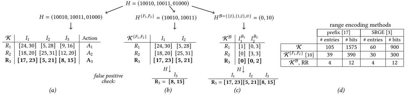
Figure 1: Our RR method vs. previous works: (a) original classifier \mathcal{K} whose rules consist of three 5-bit fields; (b) the representation of \mathcal{K} as in [10] exploiting rule disjointness based on two ranges; (c) the proposed RR implementing rule disjointness on three bits; (d) comparison of three different representations.
